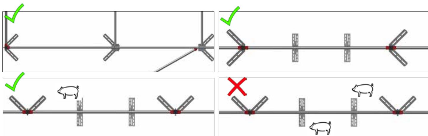
Alignment of post base plate for optimum stabilisation
