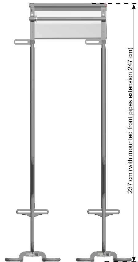
Duo rear gate - small
